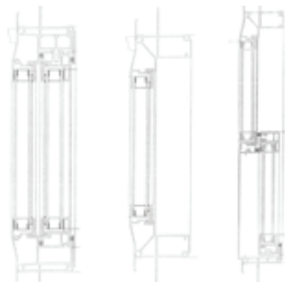
Single Slide PW SH600
